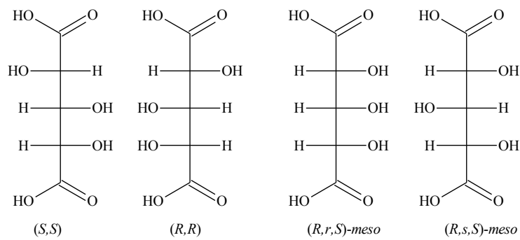
(c) Pseudoasymmetrisch centrum
